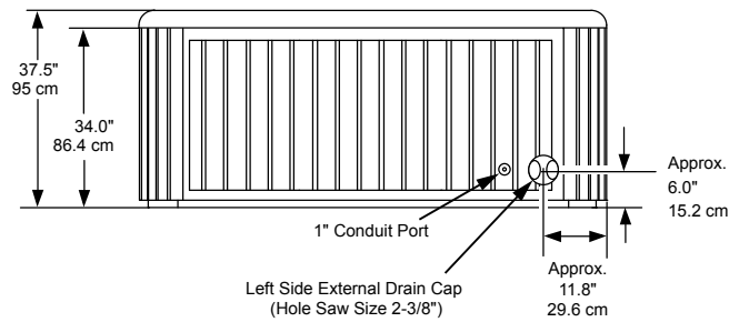
LEFT/RIGHT SIDE VIEW
