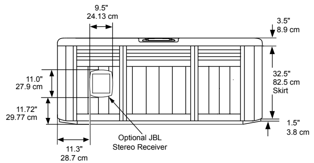
LEFT/RIGHT SIDE VIEW
